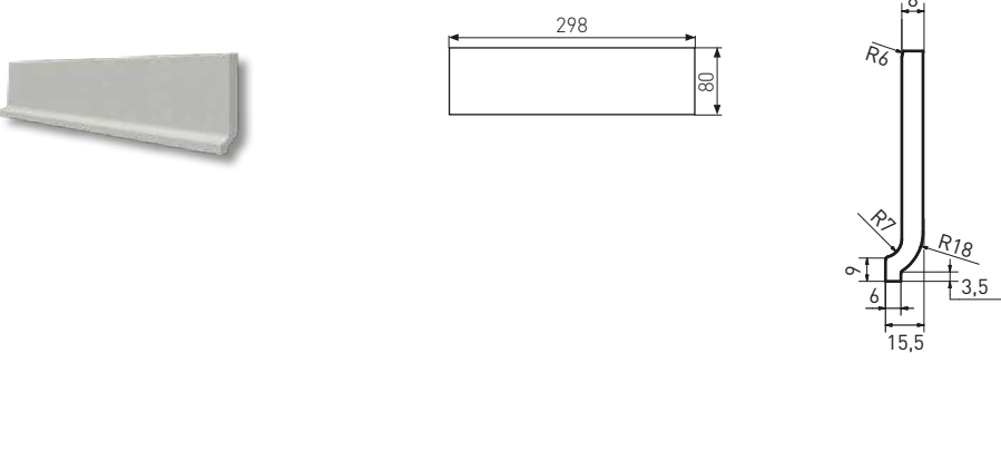
Hohlkehls sockel | cove skirting | TSPKF... | 298×80×8 mm
