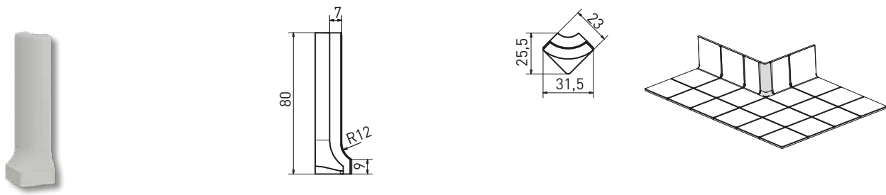
Außenecke Hohlkehlssockel | outside corner cove skirting | TSERH... | 23×80×7 mm
