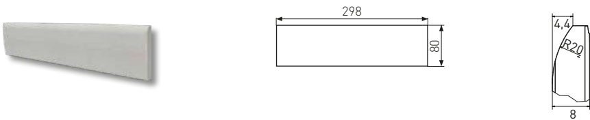
Sockel | skirting plinth | TSAKF... | 298×80×8 mm
