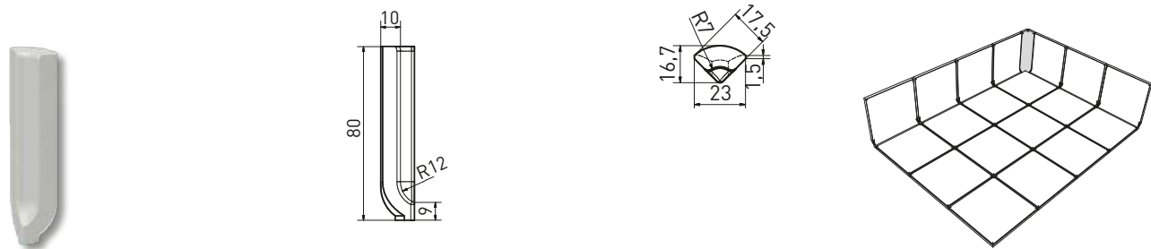
Innenecke Hohlkehlssockel | inside corner cove skirting | TSIRH... | 23×80×10 mm
