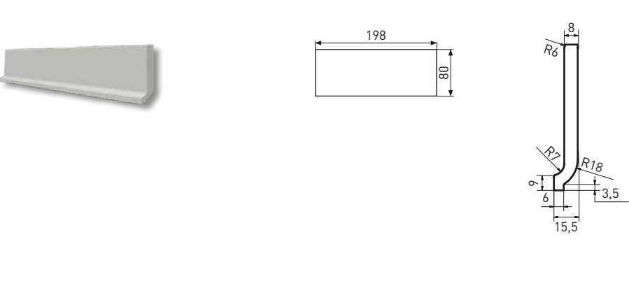
Hohlkehls sockel | cove skirting | TSPF6... | 198×80×8 mm
