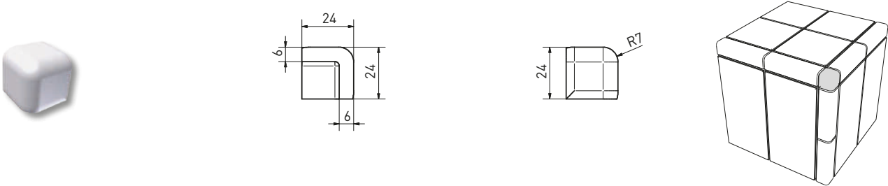
Außenecke | outside corner | GTVR4... | GTVR4F... | 24×24×24 mm
