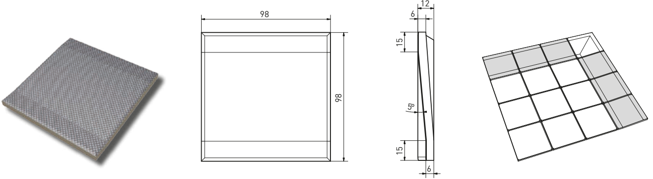
Duschtassenstein | shower piece - continuous | GTP0N... | 98×98×6 mm
