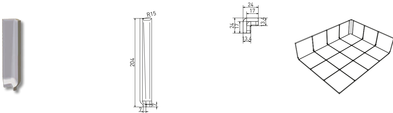
Innenecke Hohlkehlsöckel | inside corner cove skirting | GSIRI... | 24×204×7 mm
