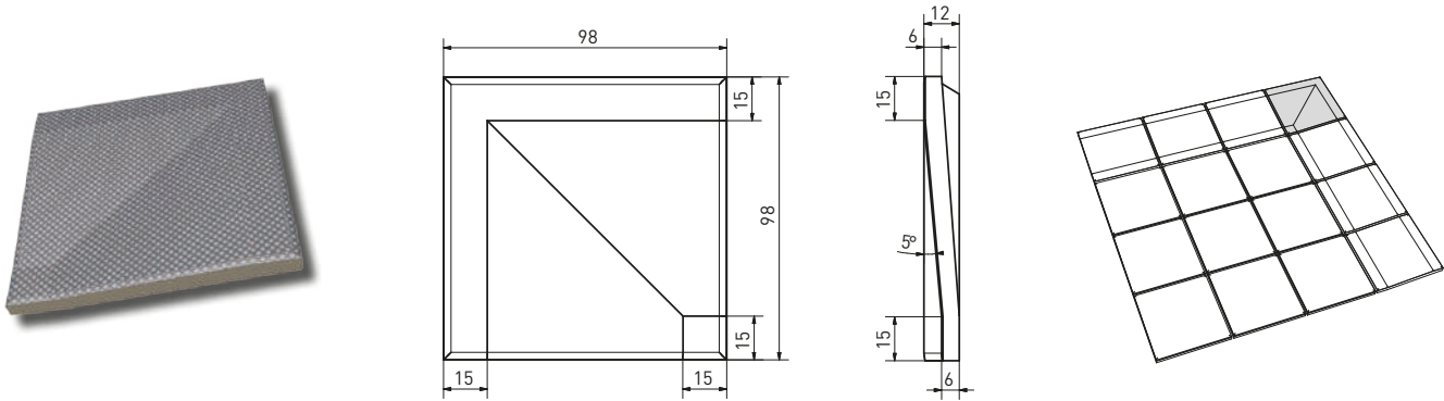
Duschtasseneckstein | shower piece - corner | GTR0N... | 98×98×6 mm
