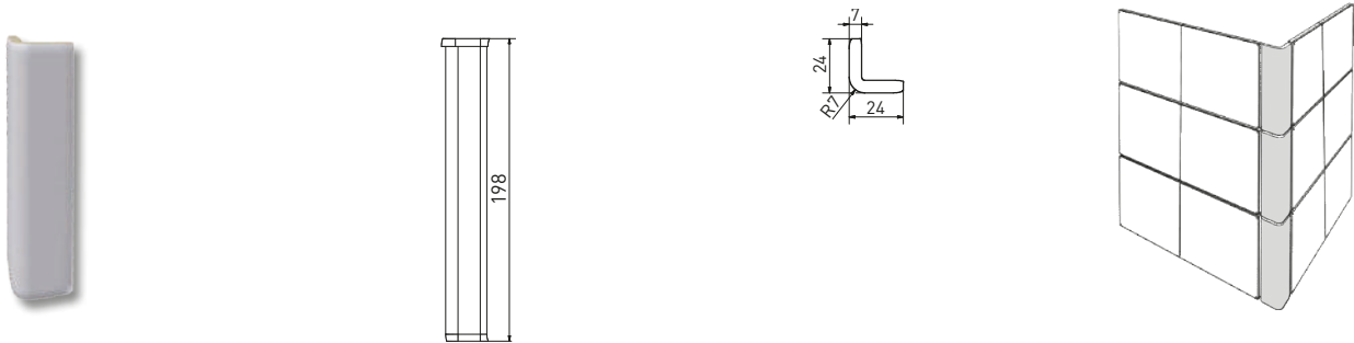
Außenkante | outside edge - shower piece | GSEAP... | GSEAPF... | 24×198×7 mm
